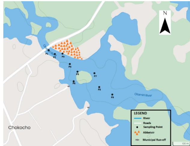
Fig. 1. A map showing the sample points in the study area of the otamiri river (source: Google Maps).
